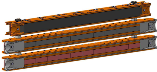
Figure 6: Present baseline for the full-jaw test at HiRadMat foresees to test a CFC jaw with integrated BPMs (top), a MoGR-base jaw (middle) and a CuCD jaw (bottom). Courtesy of L. Gentini.
