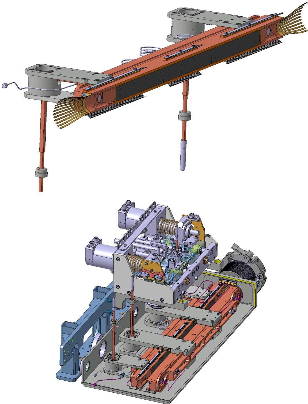
Figure 3 – Drawing of one of the TCLD jaws (top), including RF fingers, cooling pipes and BPMs, and the two jaws installed on the table (bottom). Courtesy of L. Gentini.
