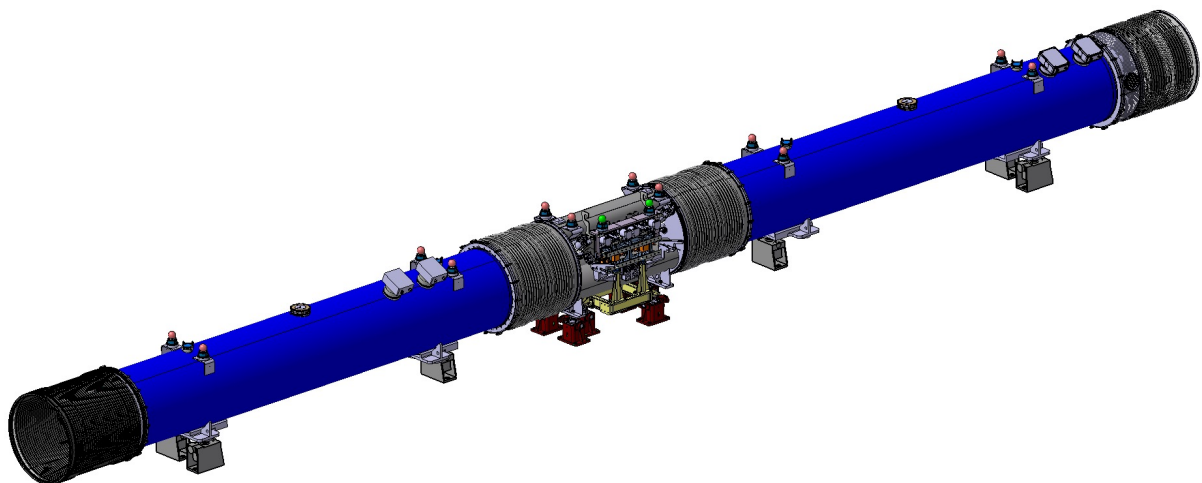
Figure 7 – A 3D drawing of the two 11T dipoles, with the collimator assembly installed in the middle.
