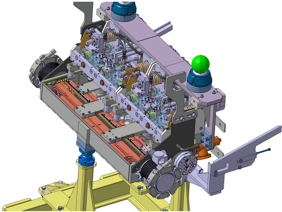
Figure 4 — 3D drawing of the TCLD jaws, integrated in the tank. Courtesy of L. Gentini.
