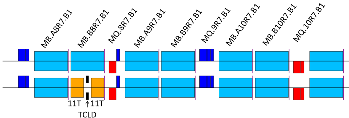
Figure 1 —Schematic layout of the B1 sequence on the right side of IR7 for the pre-LS2 installation (top row) and the proposed post-LS2 installation (bottom row), where MB.B8R7.B1 has been replaced by the assembly of two 11 T dipoles and one TCLD collimator. The layout on the left side of IR7 is fully symmetric. Courtesy of P. Hermes.
