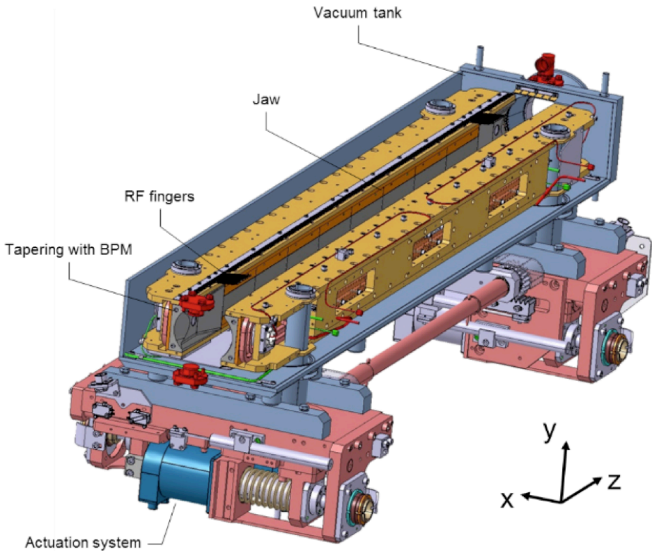
Figure 1 — 3D view [5] of the TCSPM collimator, showing an extremity of the jaw with the embedded BPM, the “third” BPM for orbit measurements in the plane orthogonal to the collimation plane, and the new tapered transitions made of MoGr.
